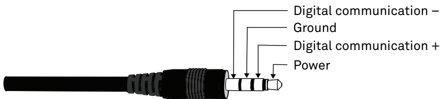
Figure 6 Stereo plug connector
