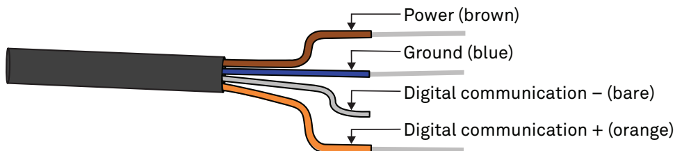
Figure 7 Pigtail wiring
