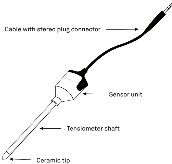
Figure 10 TEROS 31 sensor
